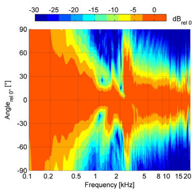
Horizontal directivity isobars
